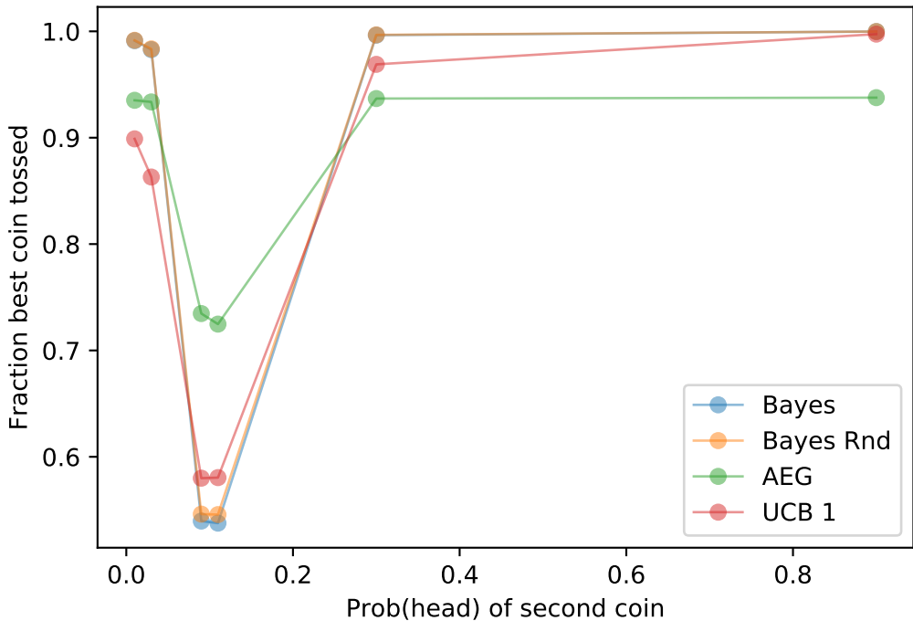
Performance after 10000 tosses
