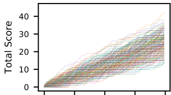
Bayes
