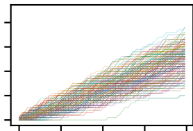
Bayes Rnd
