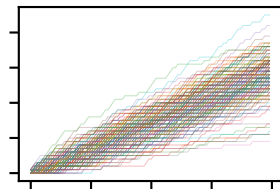
Bayes Exp
