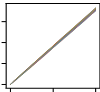
Bayes Rnd
