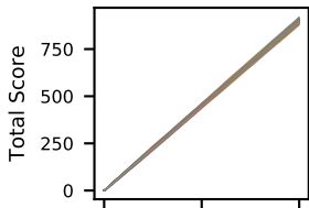
Bayes
